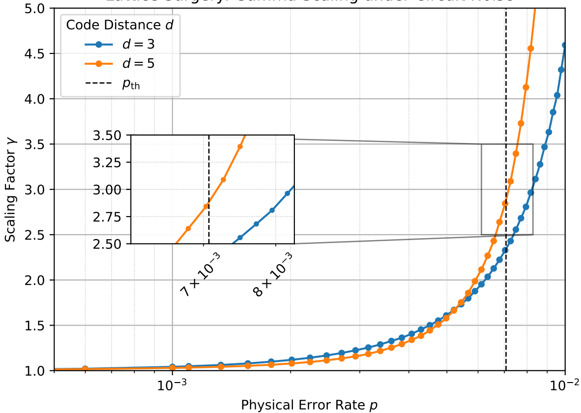
Lattice Surgery: Gamma Scaling under Circuit Noise
